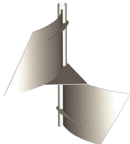
Sulzer Contour™ mixer wing pair for static mixing tasks in flue gas applications
