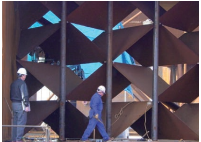
Installation of a Sulzer SMV™ mixer with Ammonia Injection Grid
