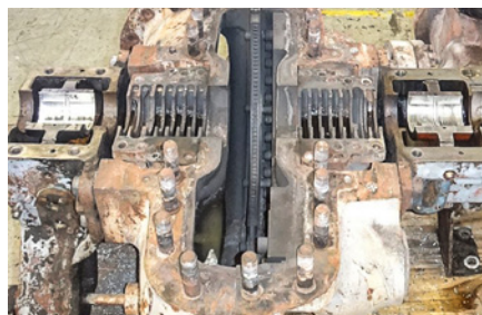
Case and nozzle repairs.
