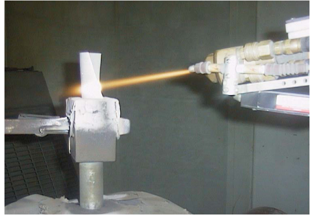
Figure 3. GE F5 Row 1 turbine blade being coated with H16
