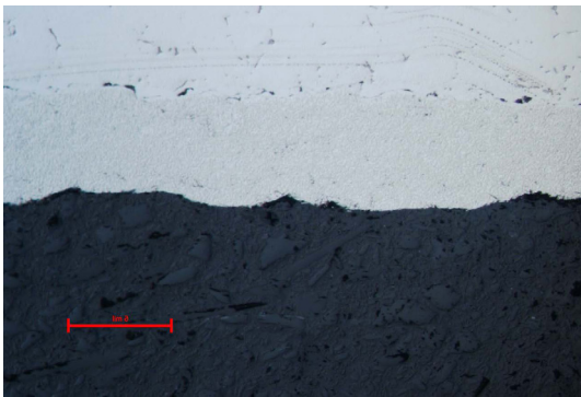
Figure 2. 200X cross section photomicrograph of H16
