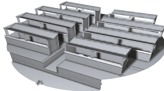
Chimney trays
