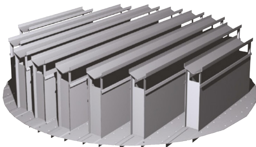
Collector-distributor systems/Vapor distributor
